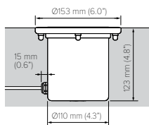
Direct Burial
