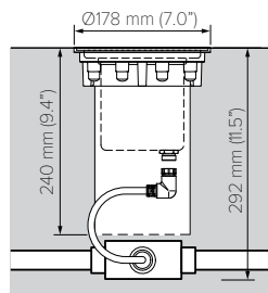
Pre-Installation
